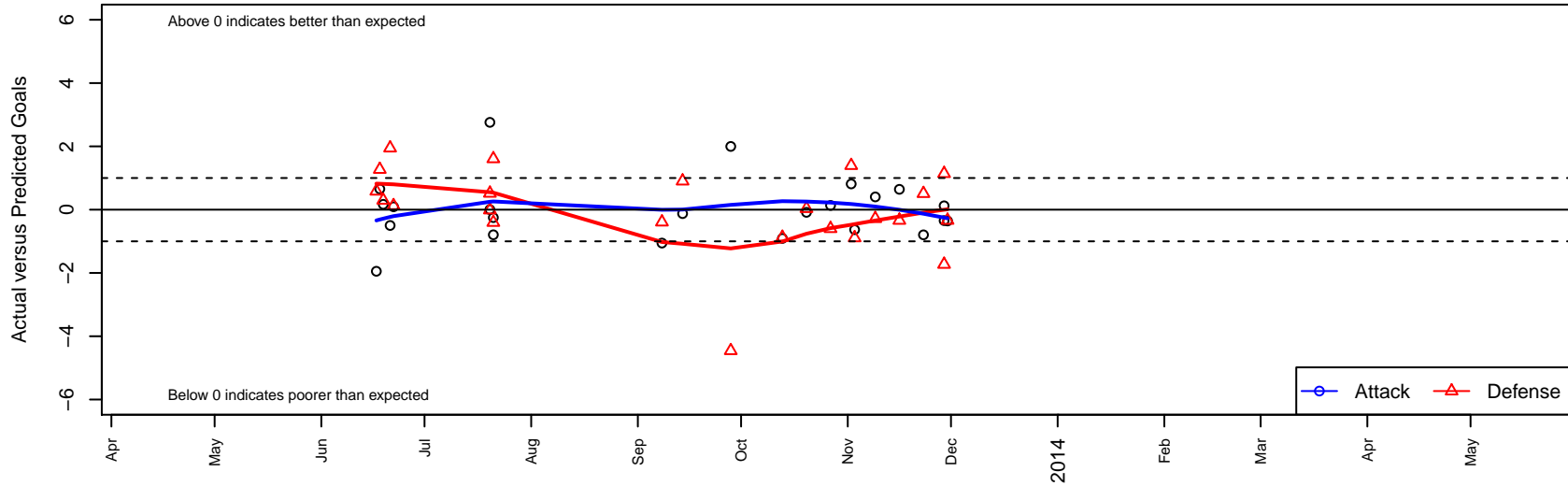
Pateadores Academy B97 Dots are actual minus expected GF (blue circles) and GA (red triangles). Blue line is smoothed change in attack strength. Red is smoothed change in defense strength.
